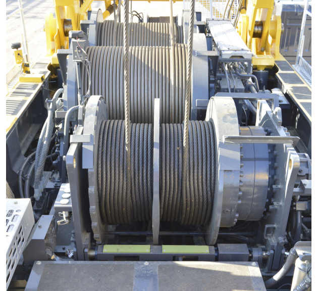
View towards the front of the machine : W1, H2 and H1 drums
